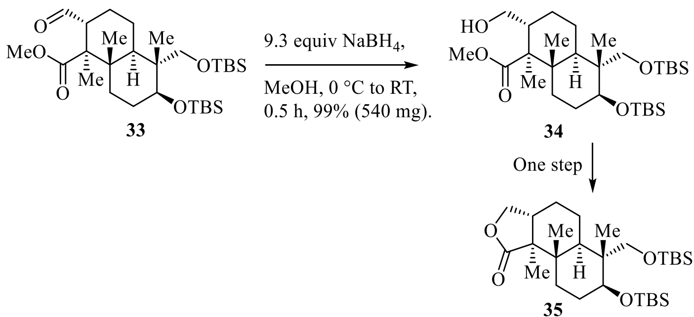
SCHEME 28
