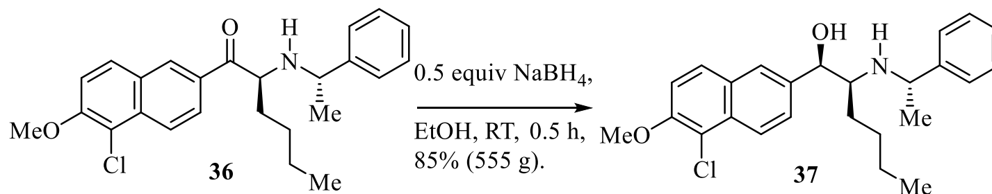
SCHEME 29
