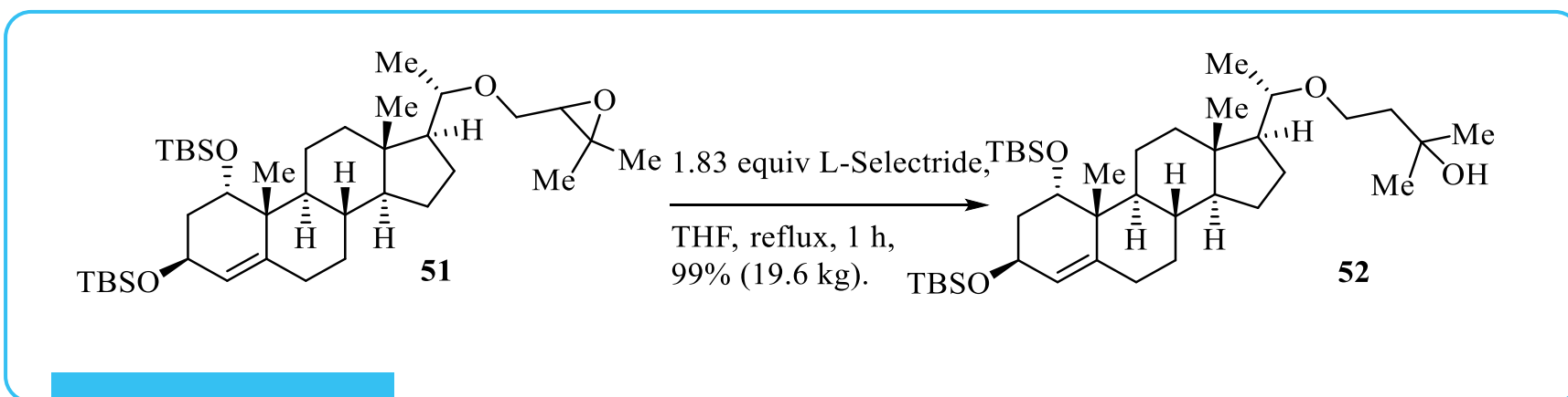
SCHEME 40
