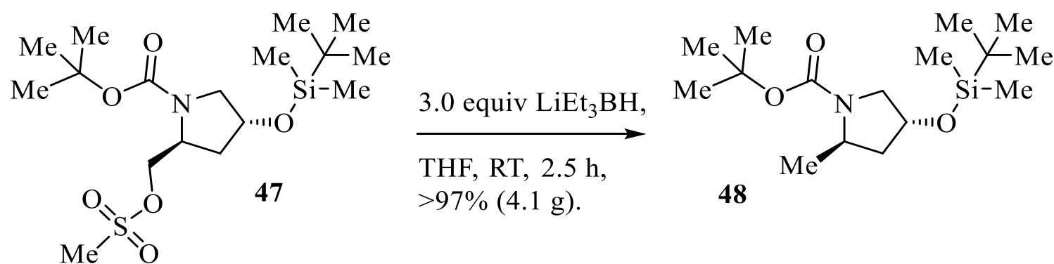
SCHEME 38
