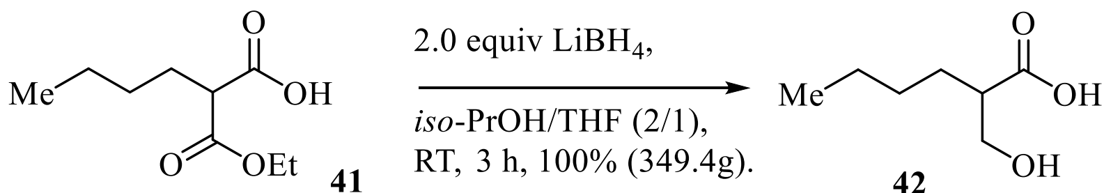
SCHEME 34
