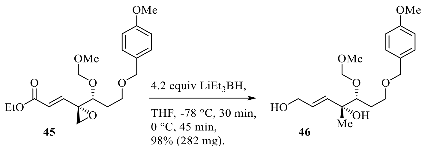
SCHEME 37
