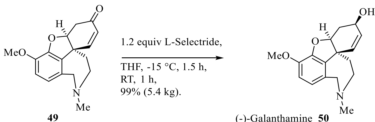
SCHEME 39
