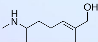
isomethptene-OH (8)
