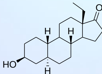
18-methyl-nortestosterone-M2 (18-methyl-3 \beta -hydroxy-5 \alpha -Estran-17-one) (20)
