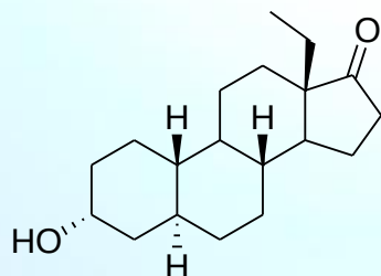
18-methyl-nortestosterone-M1 (18-methyl-3 \alpha -hydroxy-5 \alpha -Estran-17-one) (19)
