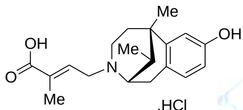
Pentazocine trans acid.HCl (13)
