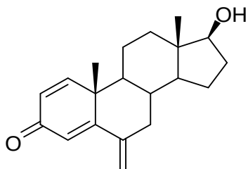
17-Dihydroexemestane (1)
