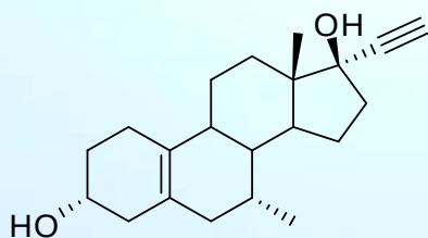
3 \alpha -hydroxytibolone (3)
