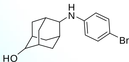
6-hydroxybromatan (6)
