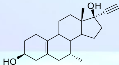
3 \beta -hydroxytibolone (4)
