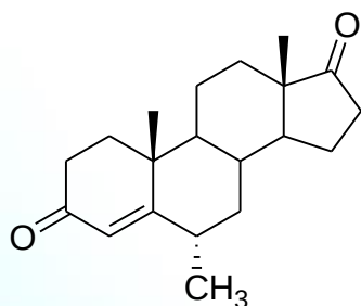
(6 \alpha )-6-methylandroster-4-ene-3,17-dione (14)
